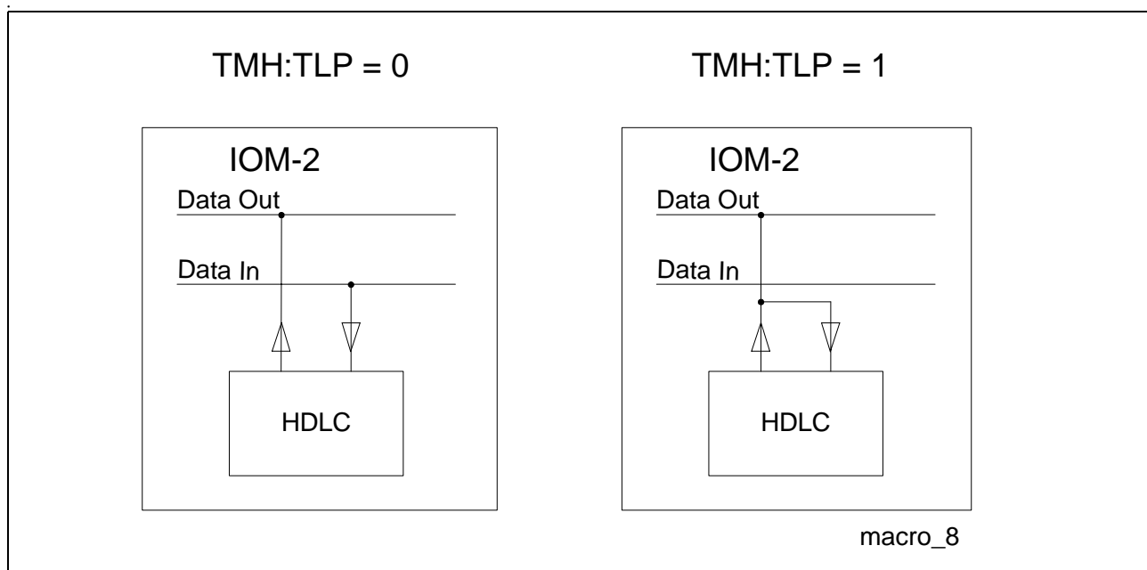
Figure 66 Layer 2 Test Loops
