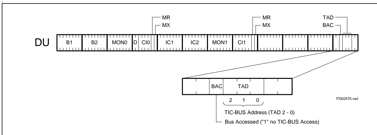
Figure 27 Structure of Last Octet of Ch2 on DU
