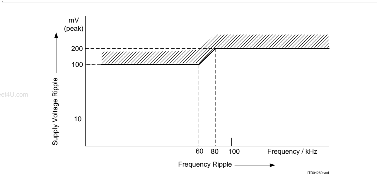
Figure 83 Maximum Sinusoidal Ripple on Supply Voltage
