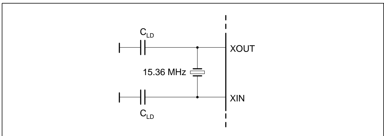
Figure 80 Crystal Oscillator
